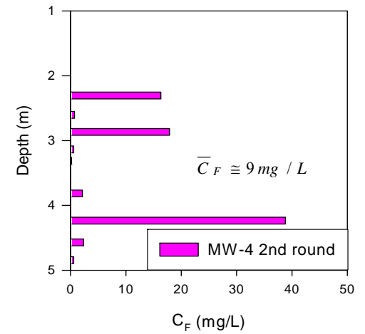
Figure 4.16 Flux-average perchlorate concentration ( C_F ) distributions in MW-1, MW-3 and MW-4 for two deployments
