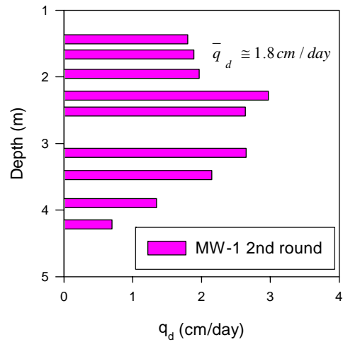
Figure 4.14 Groundwater flux ( q_d ) distribution in MW-1, MW-3 and MW-4 for two deployments
