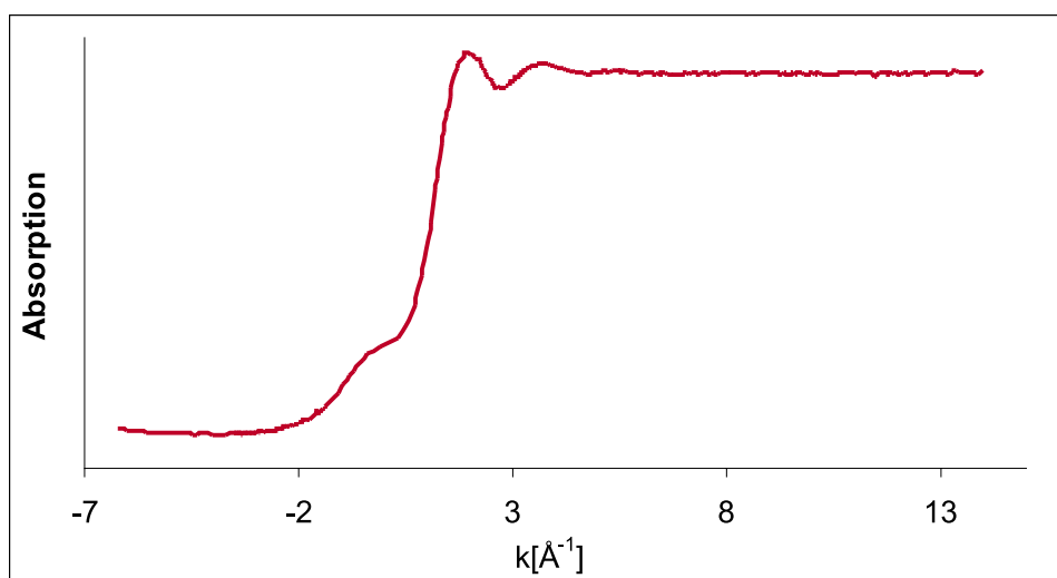
Figure C.12 k -space conversion of spectra in Figure C.11.
