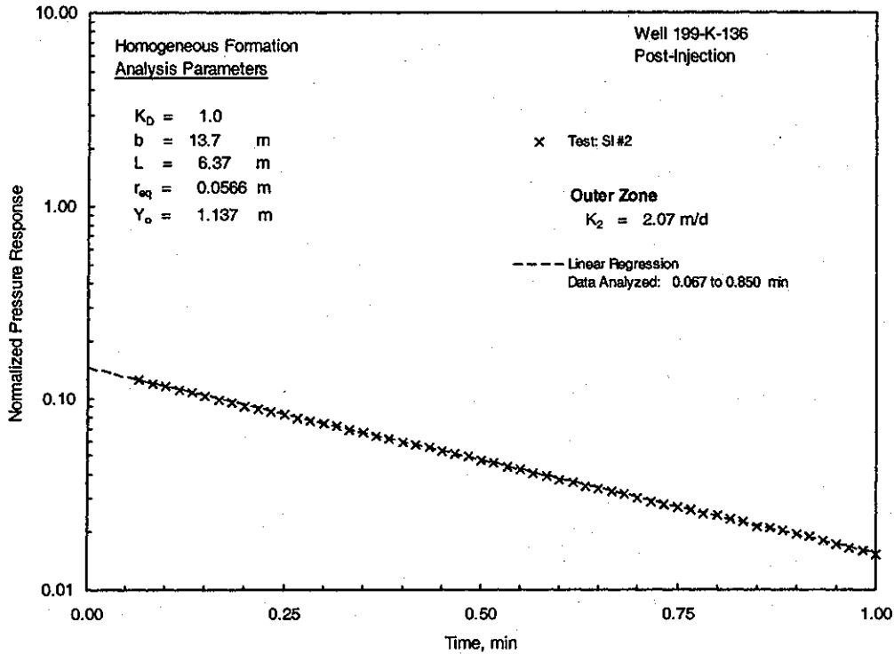
Figure D.4. Selected Post-Injection Slug-Test Analysis Plots for Injection Well K-136 [Bouwer and Rice method (top) and type-curve method (bottom)]
