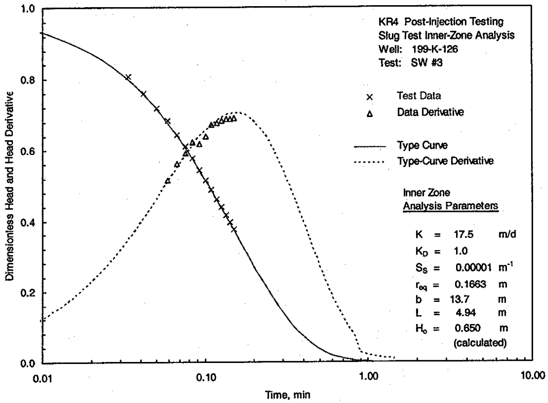
Figure D.6. Selected Post-Injection Slug-Test Analysis Plots for Extraction Well K-126: Type-Curve Inner Zone Analysis
