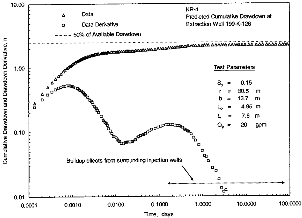
Figure 5.2 Cumulative Drawdown and Drawdown Derivative Plot for Extraction Well 199-K-126: Extraction Rate = 20 gpm (75.7 L/min)
