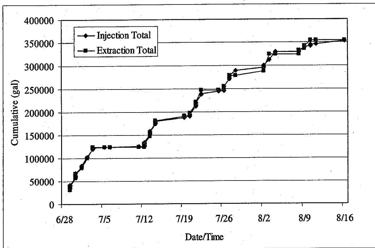
Figure 4-6. Plot of Cumulative Volume of Groundwater Extracted and Injected During the Treatability Test.
