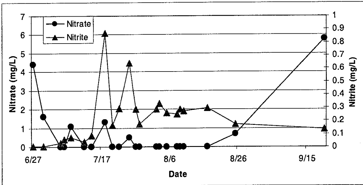
Figure 4-3. Nitrate and Nitrite Concentrations in Well 199-K-126.
