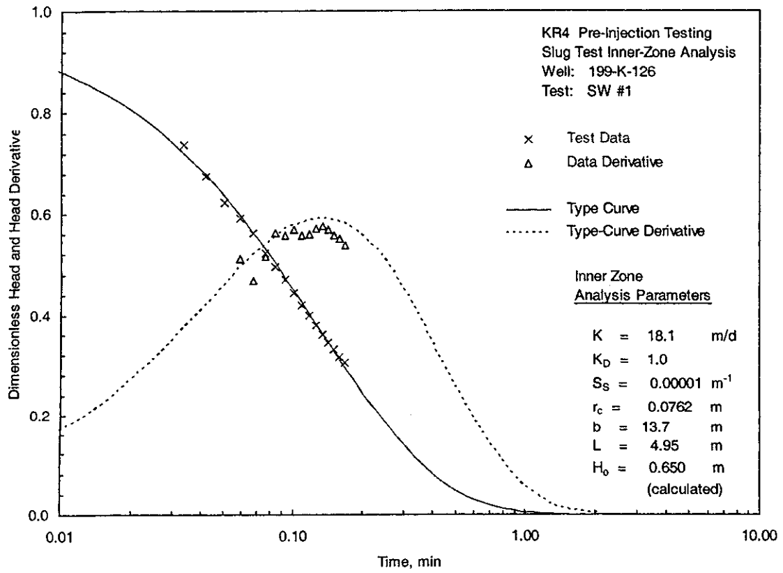
Figure A.6. Selected Pre-Injection Slug-Test Analysis Plots for Extraction Well K-126; Type-Curve Inner Zone Analysis
