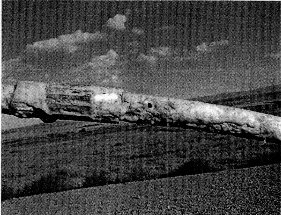
Figure C.2. Adhering Reactant Solution on Injection Line Retrieved from a KR-4 Injection Well
