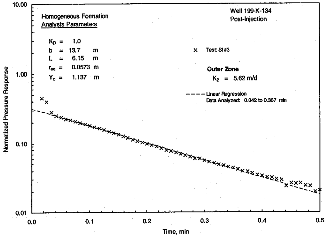
Figure D.2. Selected Post-Injection Slug-Test Analysis Plots for Injection Well K-134 [Bouwer and Rice method (top) and type-curve method (bottom)]
