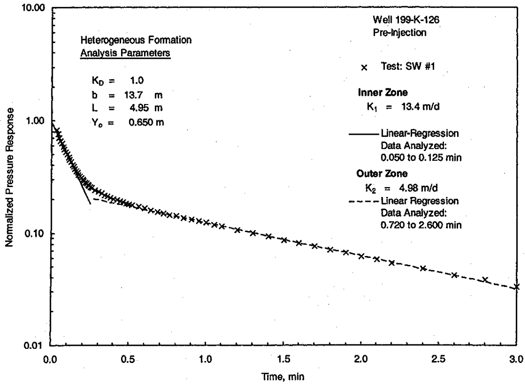
Figure A.5. Selected Pre-Injection Slug-Test Analysis Plots for Extraction Well K-126 [Bouwer and Rice method (top) and type-curve method (bottom)]
