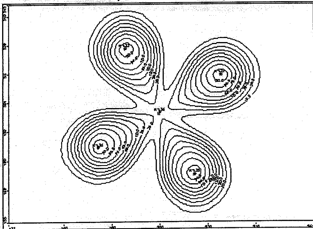
Figure 5.8 View of Areal Extent of Polysulfide Solution Following Multi-Well Circulation
