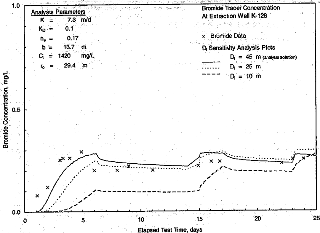
Figure 5.7 Numerical Sensitivity Analysis: Affect of Longitudinal Dispersivity, D_L
