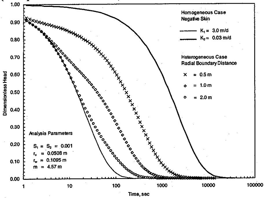
Figure 3.2 Predicted Slug-Test Response: Negative Finite-Thickness Skin Conditions (from Spane and Newcomer 2003)
