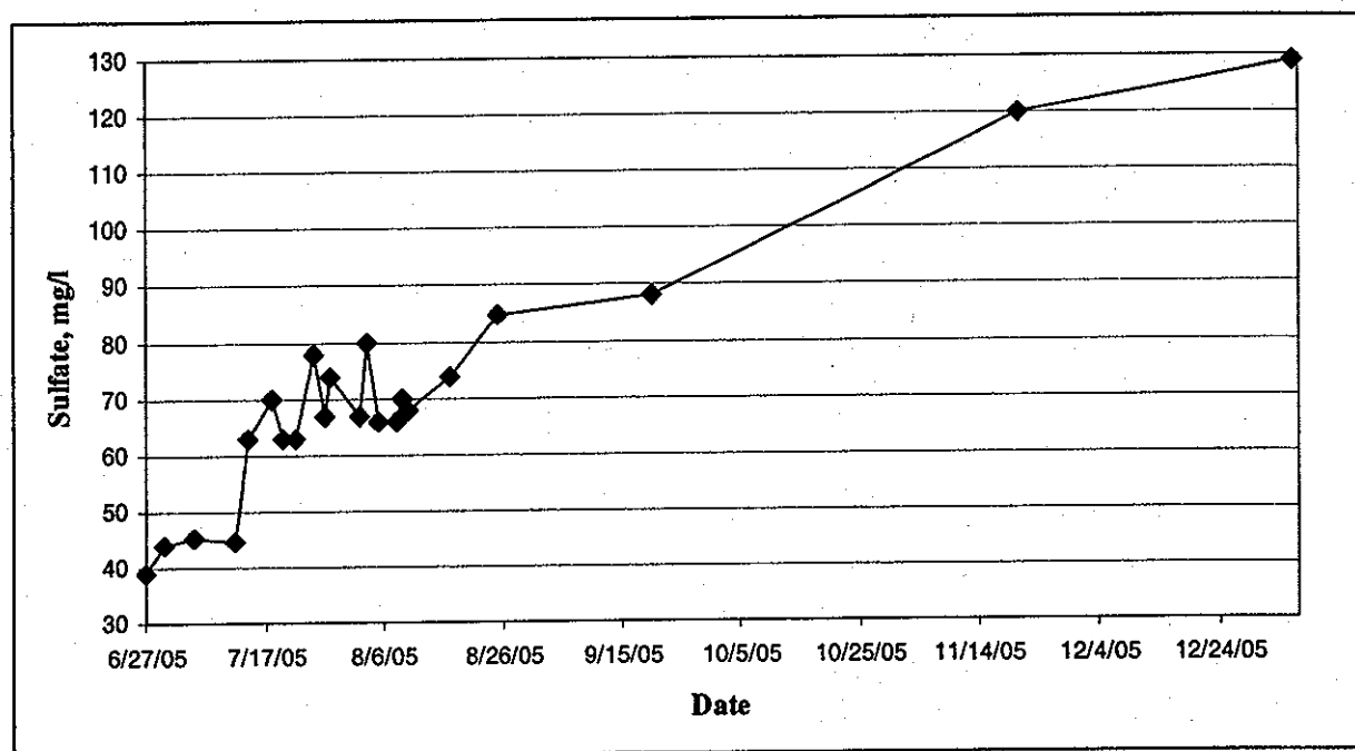
Figure 4-4. Sulfate Concentrations in Well 199-K-126.
