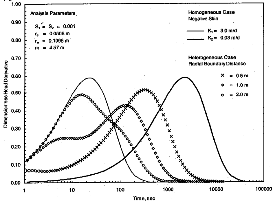
Figure 3.3. Slug-Test Derivative Response: Negative Finite-Thickness Skin Conditions (Spane and Newcomer 2003)
