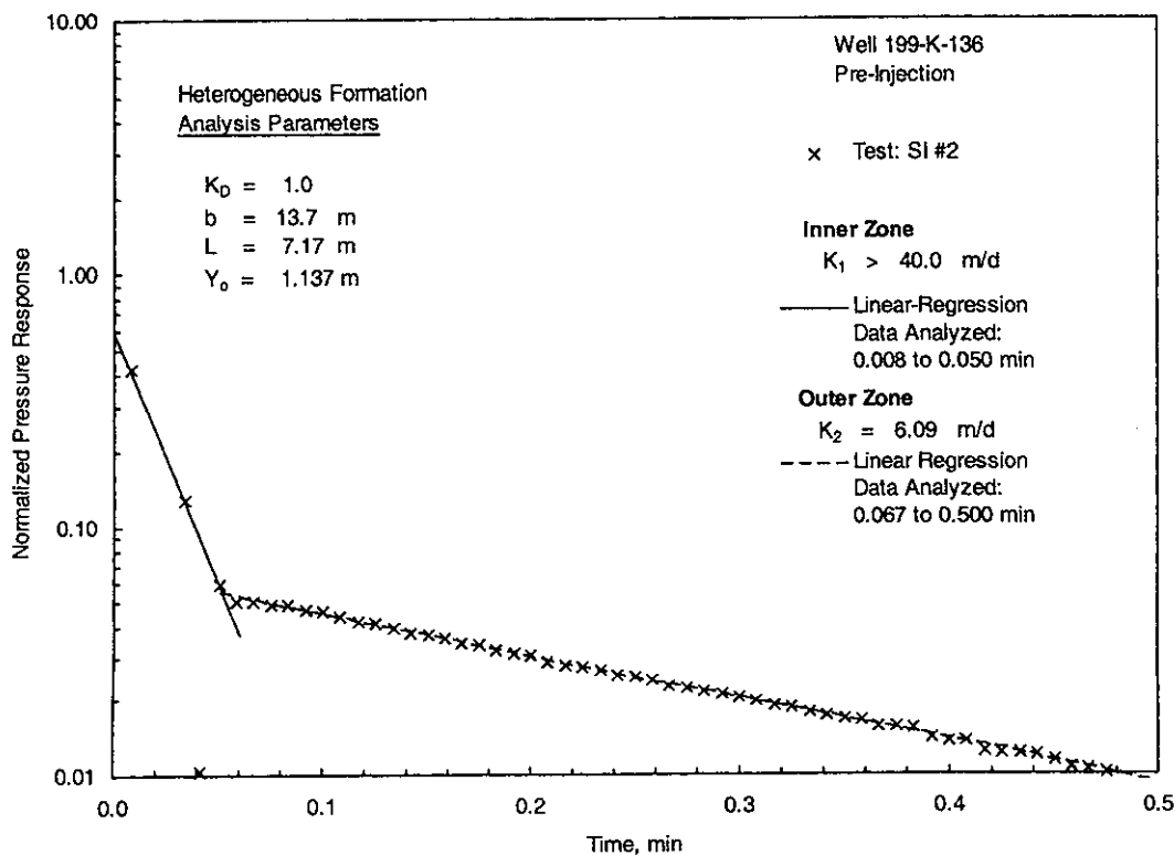
Figure A.4. Selected Pre-Injection Slug-Test Analysis Plots for Injection Well K-136 [Bouwer and Rice method (top) and type-curve method (bottom)]
