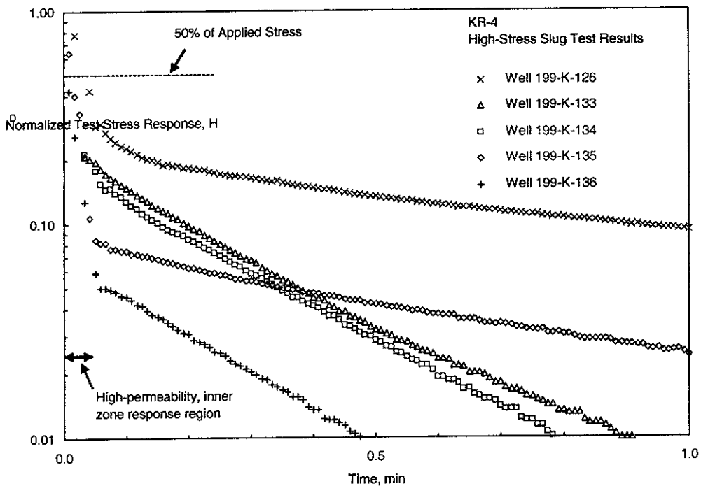
Figure 4.1. Composite Comparison of Pre-Injection Slug Test Responses at KR-4 Test Wells
