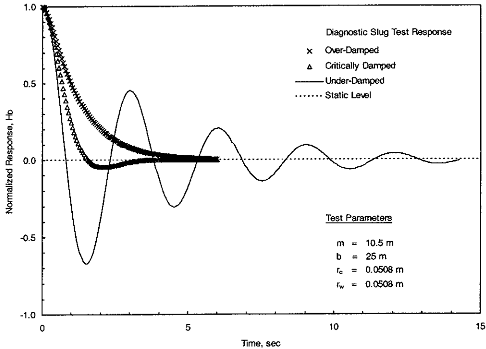
Figure 3.1. Diagnostic Slug Test Response (from Spane and Newcomer 2003)
