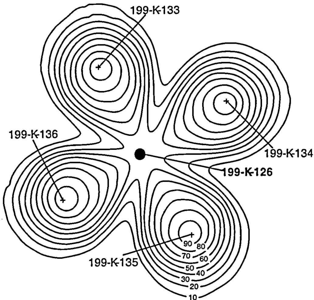
Figure 1-3. Areal Extent of Modeled Percent Concentration of Calcium Polysulfide for 100-KR-4 Treatability Test. (Further details in Appendix A.)
