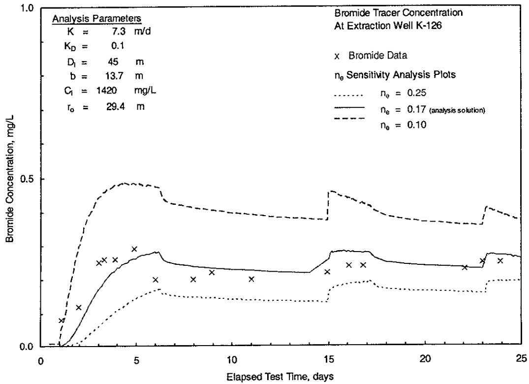
Figure 5.6 Numerical Sensitivity Analysis: Affect of Vertical Anisotropy, K_D
