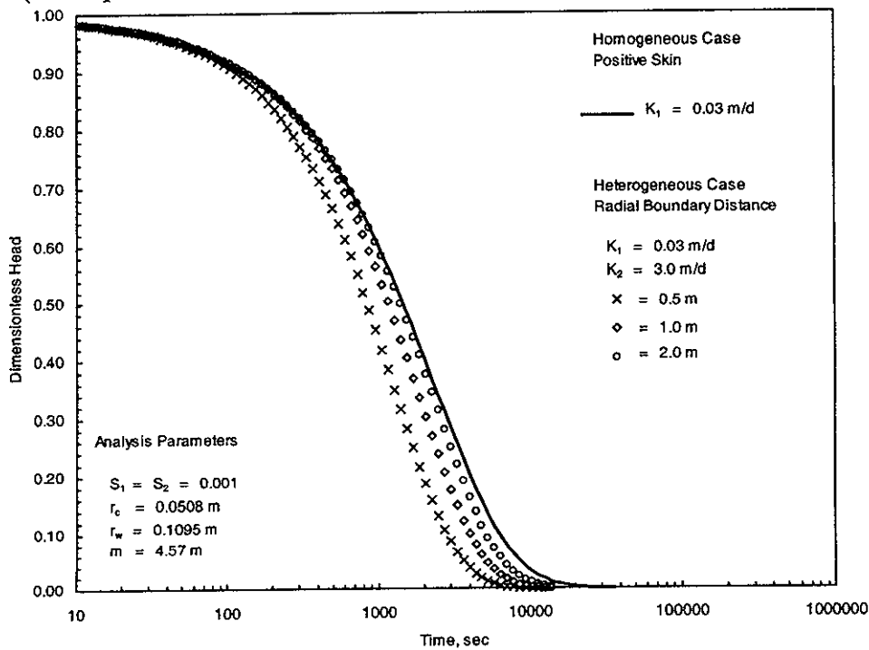
Figure 4.1. Composite Comparison of Pre-Injection Slug Test Responses at KR-4 Test Wells
