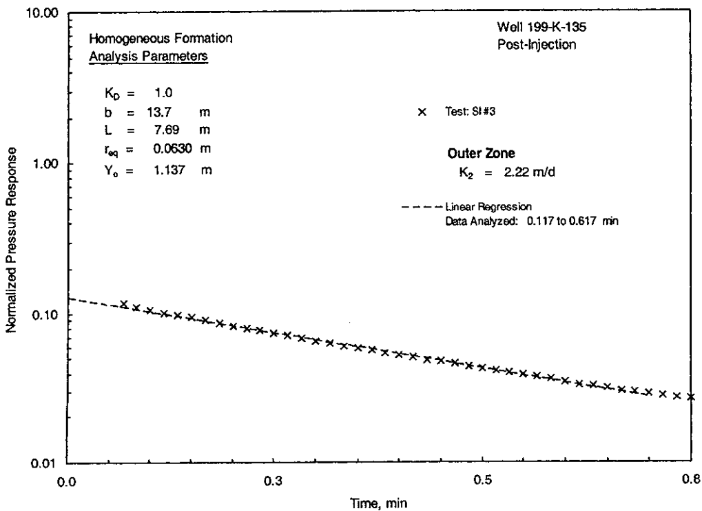
Figure D.3. Selected Post-Injection Slug-Test Analysis Plots for Injection Well K-135 [Bouwer and Rice method (top) and type-curve method (bottom)]
