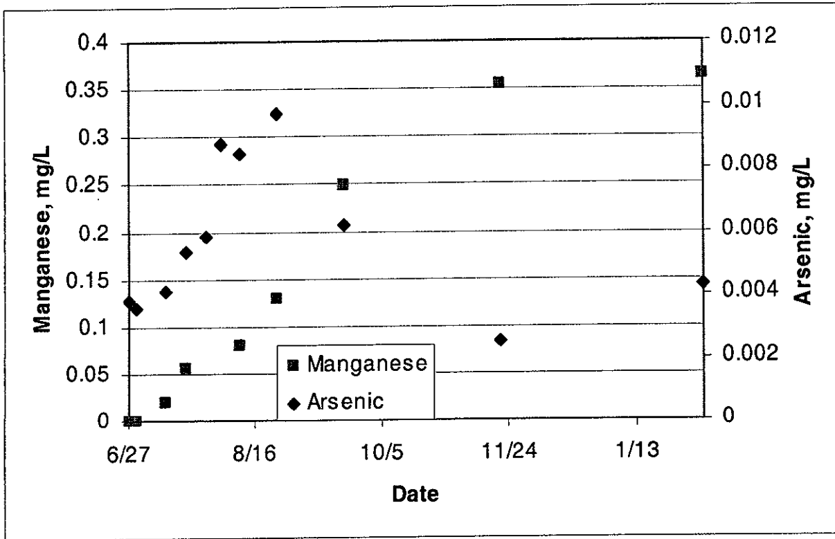
Figure 4-5. Manganese and Arsenic Concentrations in Well 199-K-126.
