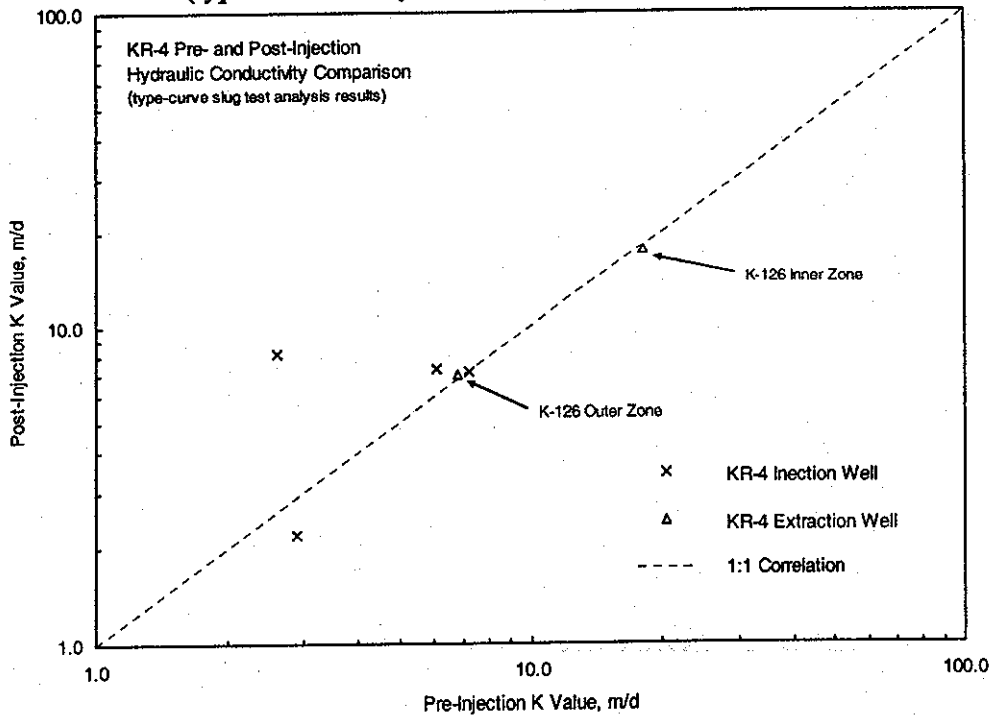
Figure 7.1 Comparison of KR-4 Test Well Pre- and Post-Injection Hydraulic Conductivity Estimates (type-curve analysis results)
