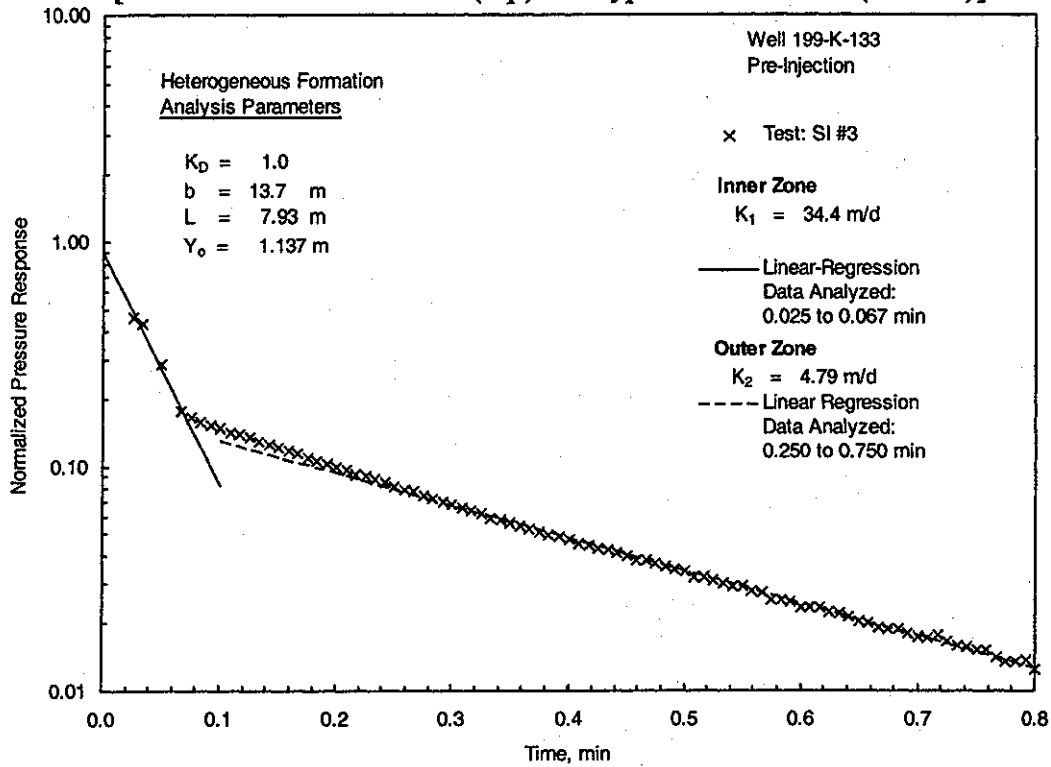
Figure A.1. Selected Pre-Injection Slug-Test Analysis Plots for Injection Well K-133 [Bouwer and Rice method (top) and type-curve method (bottom)]
