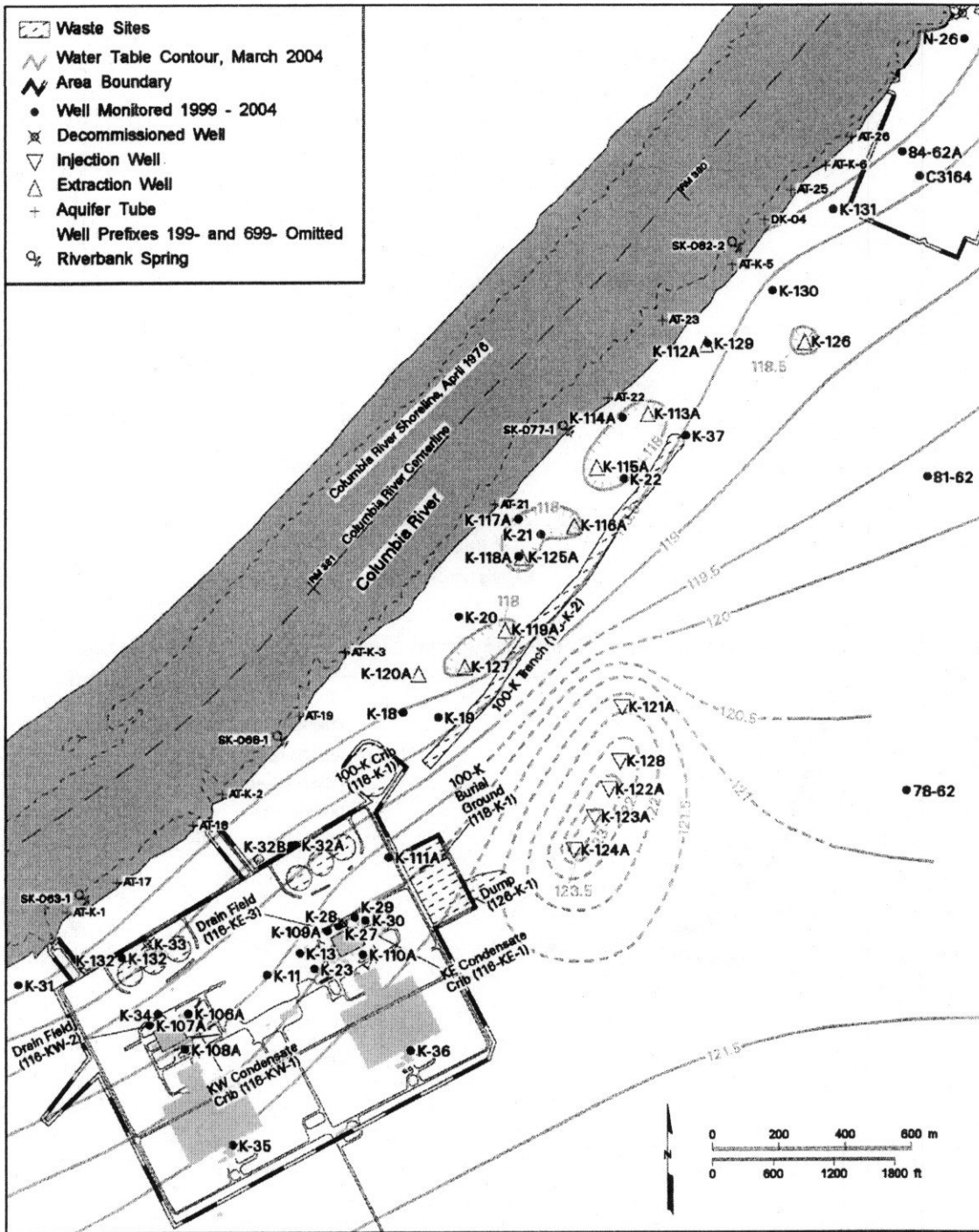
Figure 2.1. Extraction Well 199-K-129 Location Relationship to 100-K Area Facilities
