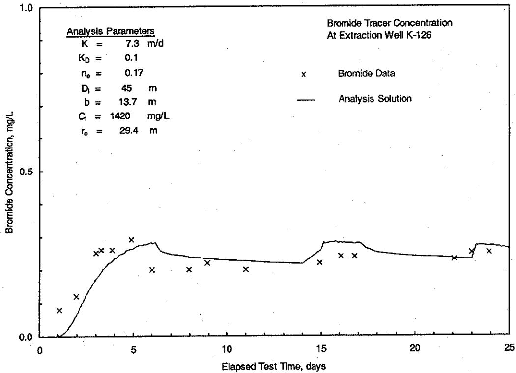
Figure 5.4 Numerical Analysis of Observed Bromide Tracer Concentrations at Well K-126
