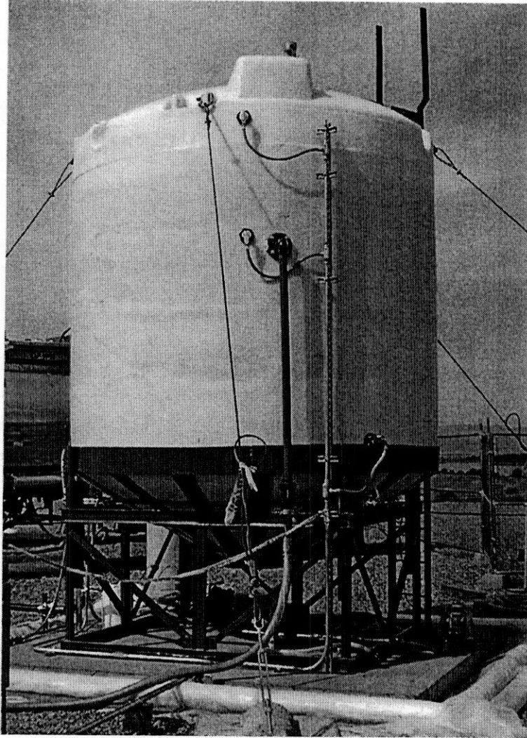
Figure 3-3. Reaction Tank used in the Treatability Test. The reacted solution was withdrawn from the tank at approximately two-thirds capacity through the 2-in. pipe.
