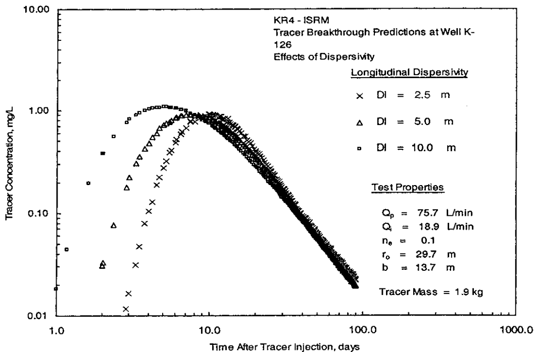
Figure B.2 Effects of Dispersivity on Predicted Tracer Breakthrough Patterns at KR-4 Extraction Well 199-K-126: D_1 = 2.5, 5, and 10 m
