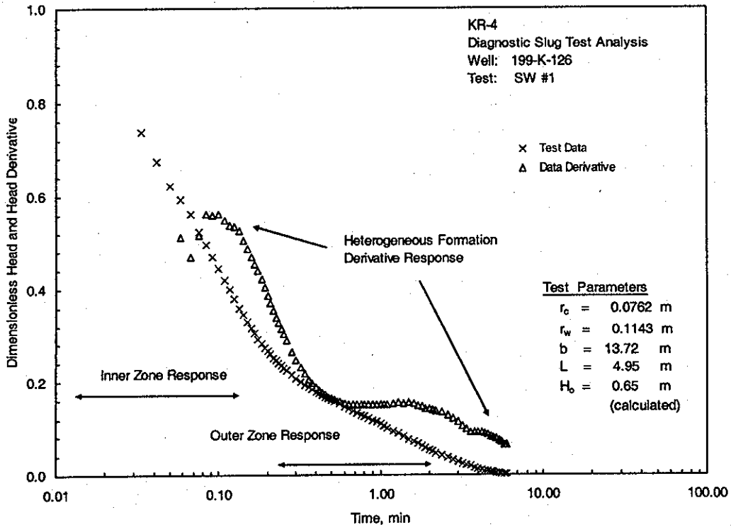
Figure 4.2. Diagnostic Slug Test Analysis – Extraction Well 199-K-126
