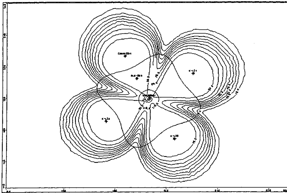
Figure B.5 Predicted Areal Reactant Isochron Map, After 3-Months of Continuous Tracer Injection ( D_1 = 5.0 m; n_e = 0.1 ; Contour Interval = 10 mg/L)
