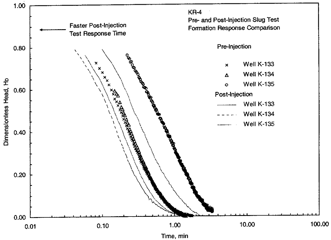
Figure 6.1 KR-4 Test Wells Exhibiting Faster Post- vs. Pre-Injection Slug Test Responses
