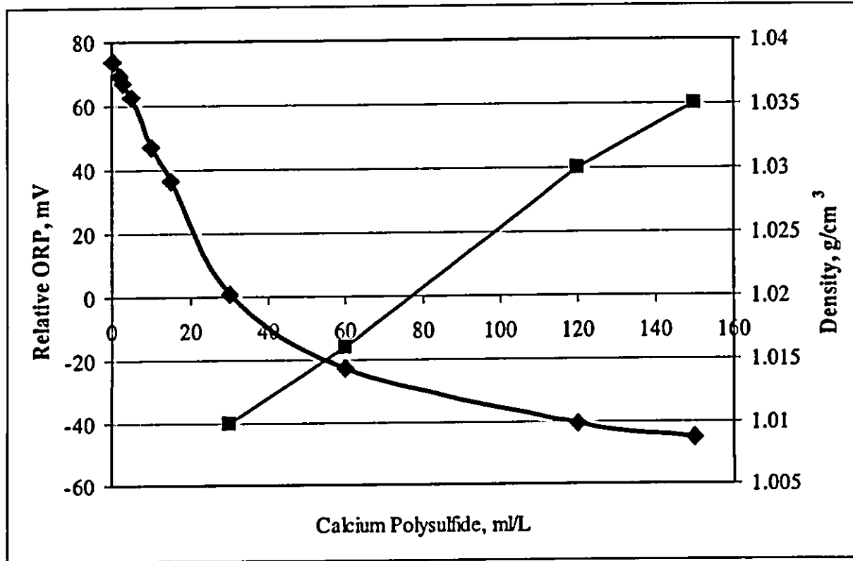
Figure 3-1. Density and Oxidation/Reduction Potential as a Function of Polysulfide Dose.
