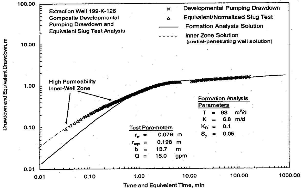
Figure 4.3. Analysis Results of Composite Well-Development Drawdown and Converted Equivalent Slug Test Response Data for Extraction Well 199-K-126
