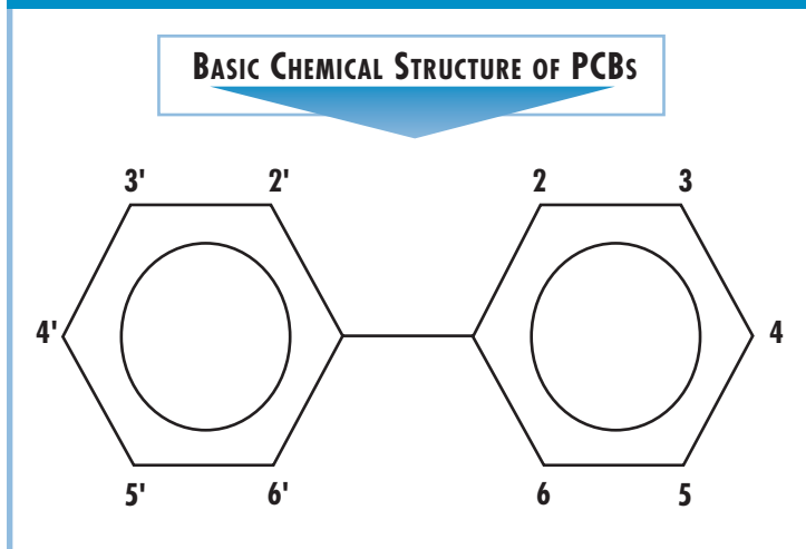
EXHIBIT 2-1: BASIC CHEMICAL STRUCTURE OF PCBs
