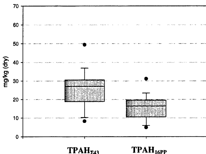
Figure 27. Box and whisker plots of TPAH Σ43 and TPAH 16PP for the 20 sediments from the study area impacted exclusively by urban background. The boxes and the whiskers represent the 25 th and 75 th and 10 th and 90 th percentiles, respectively. Outliers are BC02 (-) and SC06 (+) and these represent the 5 th and 95 th percentiles. Lines = medians.
