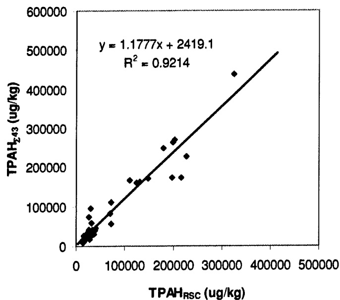
Figure 2-5. Correlation between total PAH determined by RSC (TPAH RSC ; corrected to sum of 16 priority pollutant PAH only) and by ACF (TPAH Σ43 , includes sum of 43 PAH analytes in Table 2-2). Reduced scale here does not include AW and ER surface and core samples from obvious source areas that were above the calibrated RSC range of 500,000 μg/kg.
