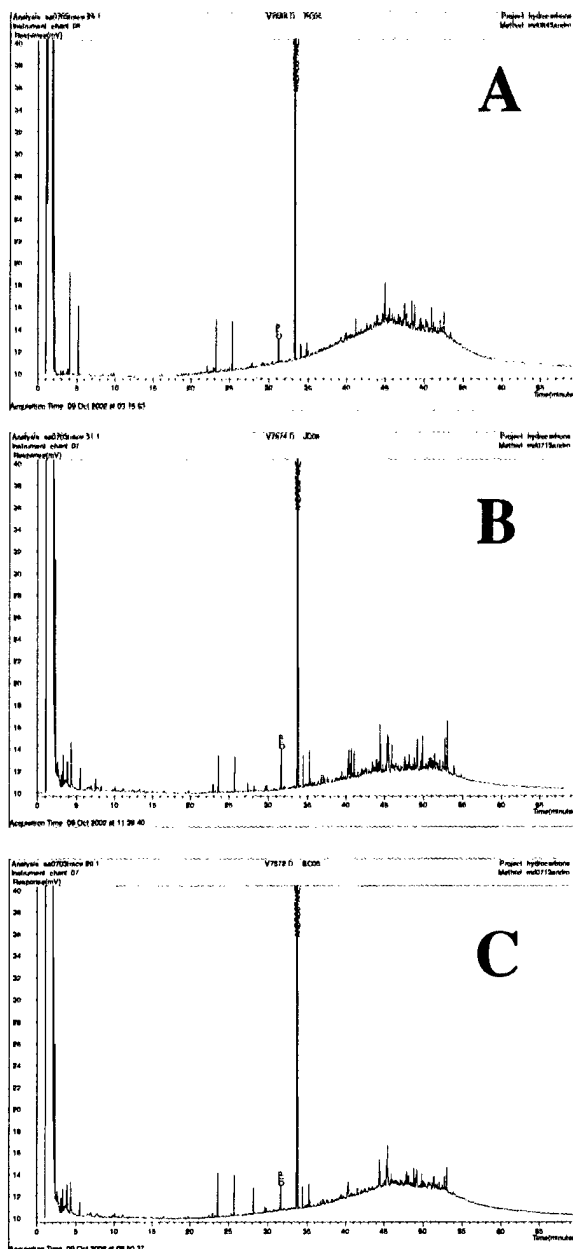
Figure 2-11. GC/FID chromatograms of extractable hydrocarbons in sediments containing hydrocarbon attributable to urban background; (A) Paradise Creek (PC05), (B) St. Juliens Creek (JC06), and (C) Scuffletown Creek (SC08). * = Int. Stand.
