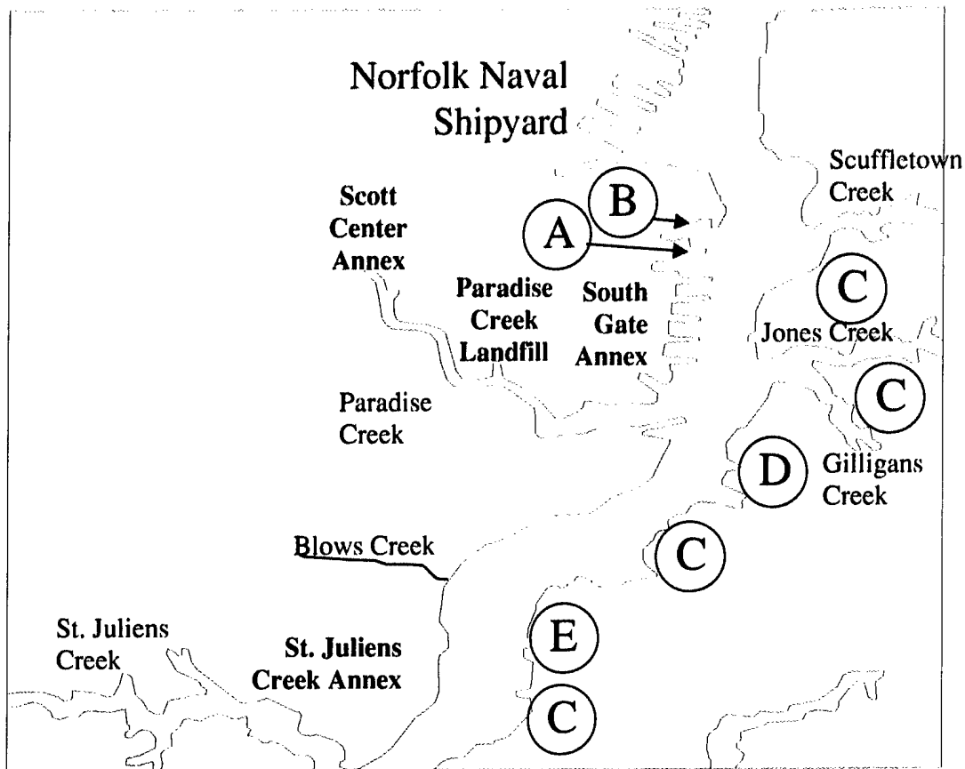
Figure 2-2. Map showing the demonstration study area along the Southern Branch of the Elizabeth River. Naval properties of interest are named and the approximate locations of commercial properties of interest include (A) Creosote Site 1, (B) Creosote Site 2, (C) multiple petroleum terminals, (D) Creosote Site 4, and (E) Creosote Site 3.
